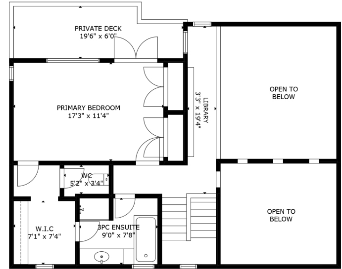
UPPER FLOOR 832 SQ FT 7'6" CEILING HEIGHT
