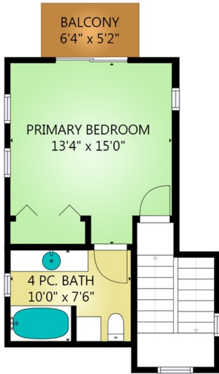
UPPER FLOOR WEST 400 SQ. FT. 11'0" VAULTED CEILING
